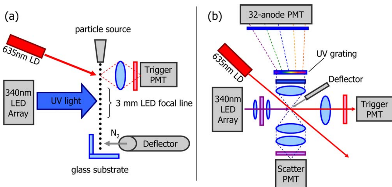
FIG. 1. Schematic of core optical system showing placement of aerodynamic deflector and substrate for sample collection. (a) Front view and (b) top view.
