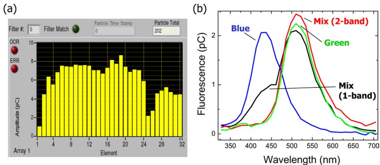
FIG. 2. (a) Portion of PC display during data acquisition showing scatter intensity detected per LED element, and (b) fluorescence spectra averaged over flagged PSL particles.
